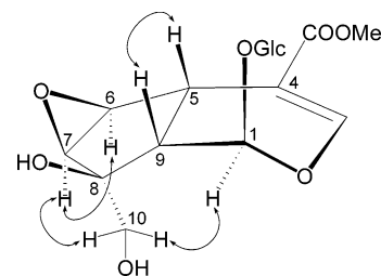
Figure 1. Selected NOESY correlations for 6 \beta ,7 \beta -epoxy-8- epi -splendoside ( 2 ).
